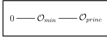
Figure 5.1: Hasse diagram for \mathfrak{sl}(3)
