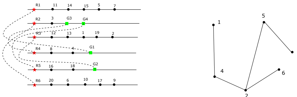
Figure 4.2. The matching on linegram in Figure 4.1 and the associated tree.
