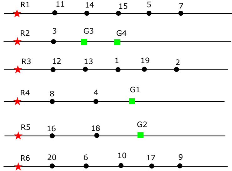
Figure 4.1. A linegram with n = 6 and g = 9 .
