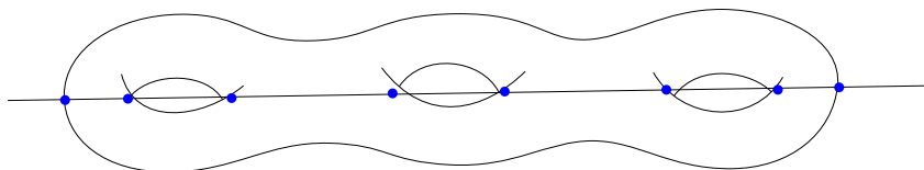
Figure 2.1. How we can try to visualize an admissible double covering of a 8-pointed curve of genus 0, resulting in a hyperelliptic curve of genus 3
