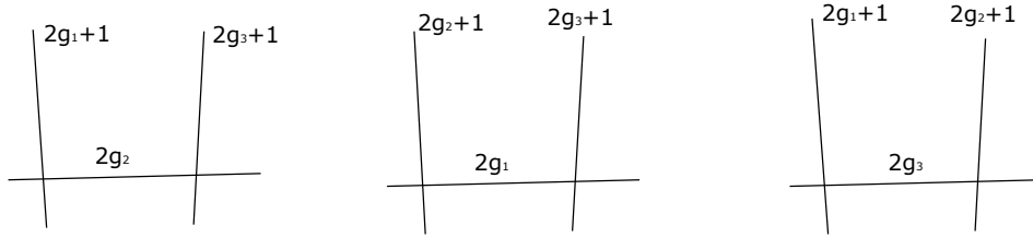
Figure 4.3. The three possible trees. The central component is different every time; we write down the number of black points on each component.
