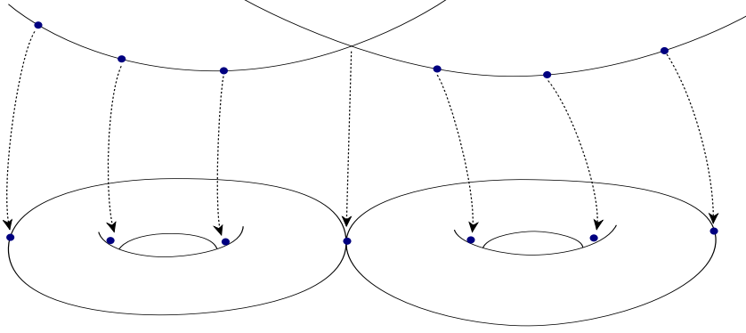
Figure 3.1. A generic point of \Delta_D when D \subset \{1, \dots, 6\} is odd
