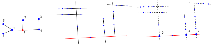
Figure 2.2. The tree associated to a product of smooth genus 0 curves, with |p(i)| on every vertex and the central vertex, and how we are going to contract it onto the central component; note that \sum |p(i)| = 20 which is greater than 9, 3 and 7.
