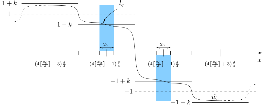
FIGURE 7. The joining transition \hat{w}_\varepsilon .
