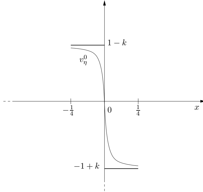
FIGURE 4. The function v_\eta^0 .
