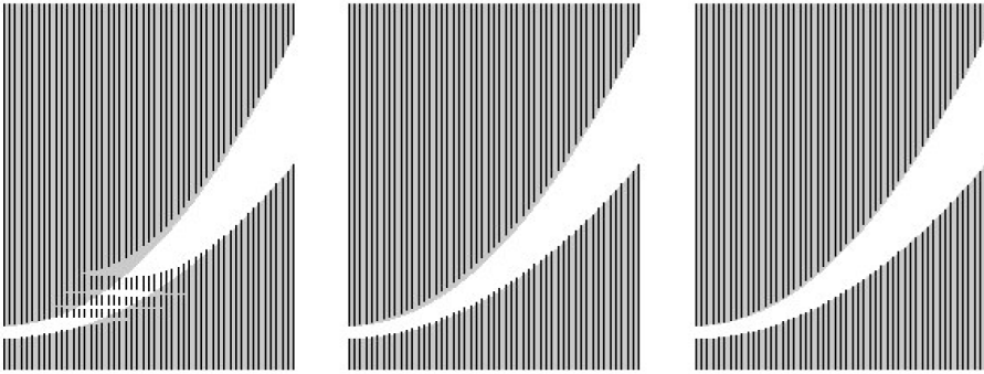
Fig. 4: (a) F(x) - in gray. Fifty cross-sections of B_{12}(F, u) - in black. (b) F(x) - in gray. Fifty cross-sections of B_{13}(F, u) - in black. (c) F(x) - in gray. Fifty cross-sections of B_{30}(F, u) - in black.
