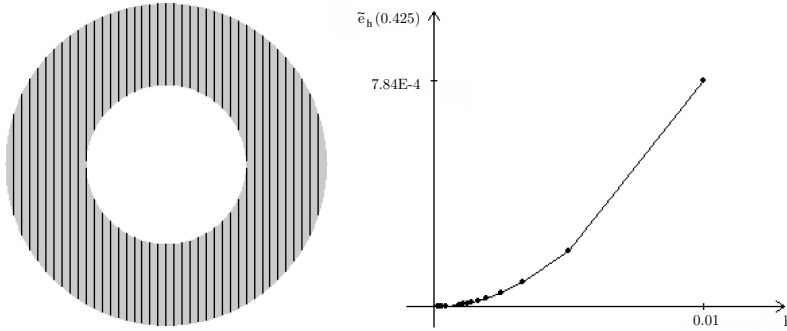
Fig. 3: (a) F - in gray. Forty cross-sections of \tilde{S}_{4, 0.01}F - in black. (b) Error between the original and the reconstructed cross-sections at x = 0.425 as function of h .
