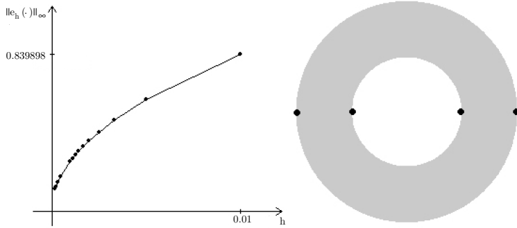
Fig. 2: (a) Maximal error between the original and the reconstructed cross-sections as function of h . (b) Points of change of topology, where the maximal error is attained.
