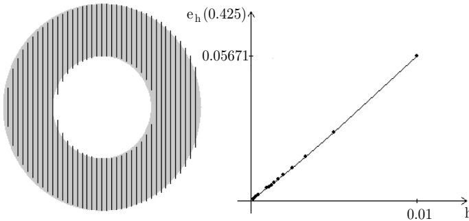
Fig. 1: (a) F - in gray. Forty cross-sections of S_{3,0.01}F - in black. (b) Error between the original and the reconstructed cross-sections at x = 0.425 as function of h .
