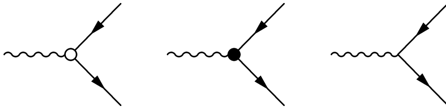
Fig 3: Graphical representation of \mathcal{A}_0 , \mathcal{A}_- and \mathcal{A}_+
