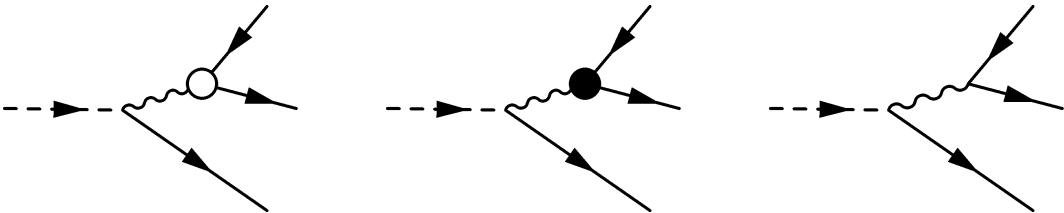
Fig 6: Graphical representation of the interactions \mathcal{T}_0^{(\mu)} , \mathcal{T}_-^{(\mu)} and \mathcal{T}_+^{(\mu)}
