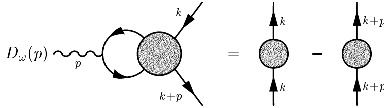
Fig 1: Graphical representation of (1.1.7)
