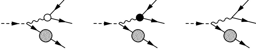
Fig 7: Graphical representation of items 1.
