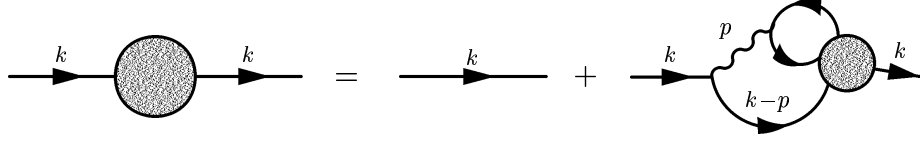
Fig 2: Graphical representation of (1.1.12)
