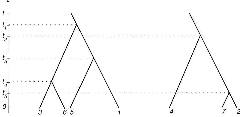
Figure 2.2: Tree graph \Gamma(2, 5) = 1, 2, 1, 3, 2 . We have also drawn a time arrow in order to associate times to the nodes of the trees: at time t_i the line j + i is “created”. Lines 1 and 2 exist for all times; they are called “root lines”.
