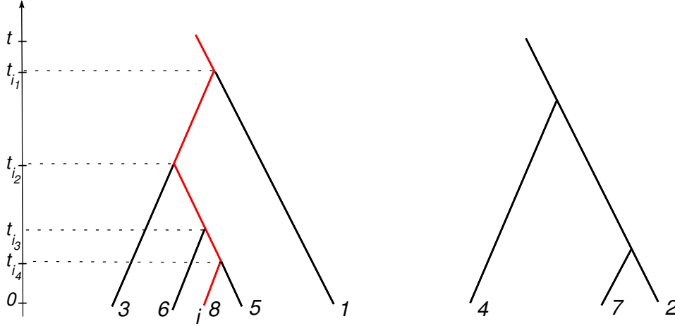
Figure 2.6: Path \mathcal{P}_i in the tree \Gamma(2, 6) , with i = 8 . The state of the particle associated to it via the BBF is called “virtual trajectory”.
