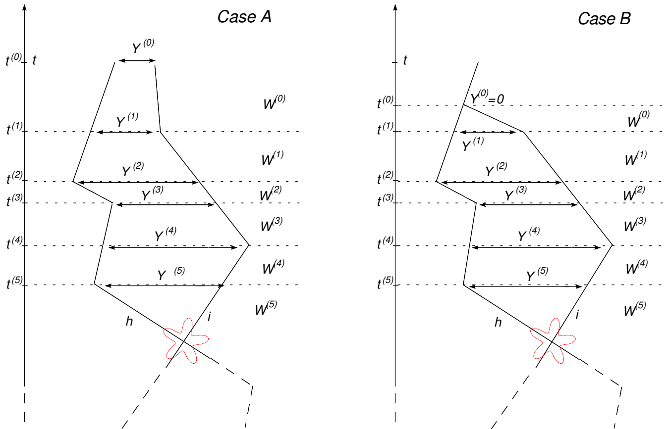
Figure 2.7: A symbolical drawing of virtual trajectories of two particles i, h in the BBF showing a \delta -overlap. Relative distances and velocities are indicated as defined in (2.8.10). In case A the two particles belong to different trees, while in case B they belong to the same.
