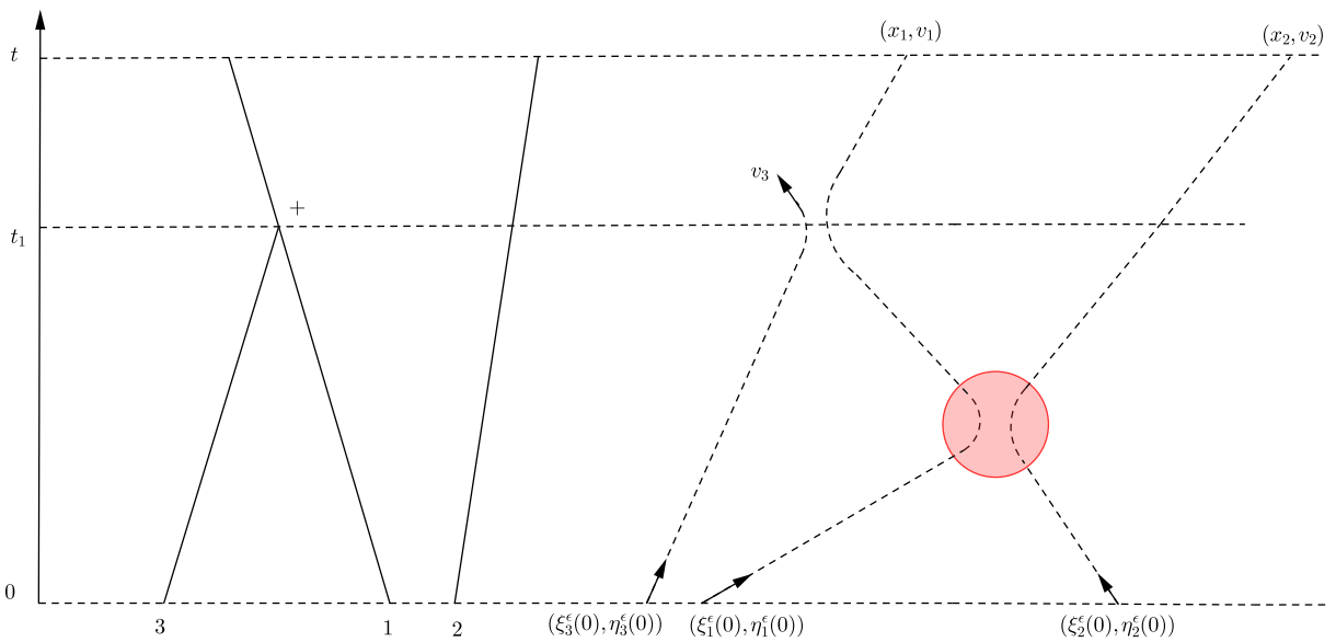
Figure 2.4: On the left, a simple case: \Gamma(j, n) = \Gamma(2, 1) = 1 . The plus sign on the node recalls that \sigma_1 = + . We want to estimate the contributions to the corresponding formula \mathcal{T}_+^\varepsilon(\mathbf{z}_2, t) , coming from the recolliding trajectories of the IBF. An example of such a trajectory is symbolically represented in the figure on the right.
