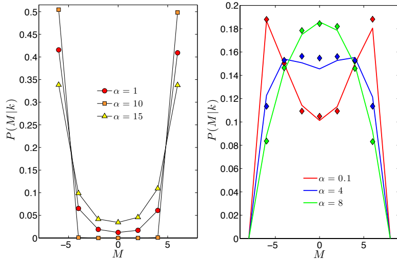
Figure 2.8: Left panel: overlap distribution P(M|k) at zero field in the over-percolated regime, for k = 6 , c = 1 and \beta = 0.8 , and different \alpha values (see legend). Right: the same distribution at \beta = 0.8 , but now for k = 6 , c = 3 , and different \alpha values (see legend). Note the different vertical axis scales of the two panels. Solid lines: theoretical predictions, calculated via the population dynamics method. Markers: results of measuring the overlap statistics in Monte-Carlo simulations of the spin system with Hamiltonian (2.53), with N = 3.10^4 . The theory predicts that here P(M|k, 0) is no longer independent of \alpha , which we find confirmed. Note that M \in \mathbb{Z} , so line segments are only guides to the eye.
