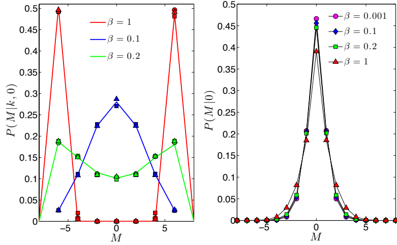
Figure 2.7: Left: degree-conditioned conditioned overlap distribution P(M|k,0) in the under-percolated regime, for k = 6 , c = 1 , and different \beta values (see legend), without external fields. Solid lines: theoretical predictions. Markers: results of measuring the overlap statistics in Monte-Carlo simulations of the spin system with Hamiltonian (2.53), with N = 3 \cdot 10^4 spins. Different symbols represent different values of \alpha , namely \alpha = 0.005 (bullets), \alpha = 0.008 (squares) and \alpha = 0.011 (triangles). The theory predicts that here P(M|k,0) is independent of \alpha , which we find confirmed. Right panel: overlap distribution P(M|0) at zero field in the under-percolated regime, for k = 6 , c = 1 and \alpha = 0.5 , and different temperatures (see legend). Note that M \in \mathbb{Z} , so line segments are only guides to the eye.
