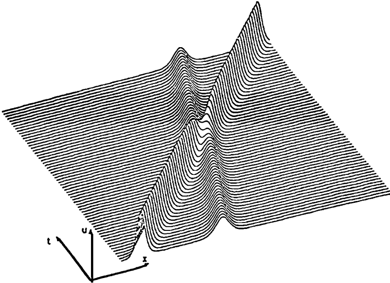
Fig. 1 Two-soliton solution of the KdV equation
