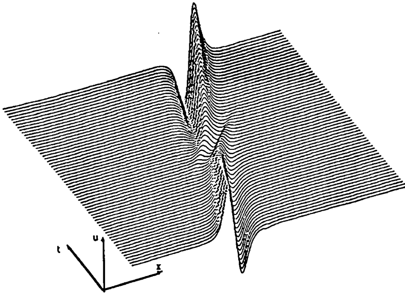
Fig. 6 Derivative of Angle-variable density of the KdV equation.
