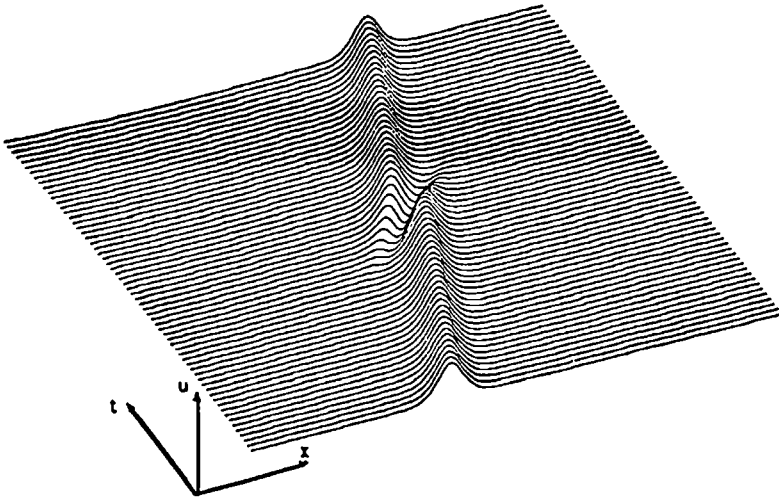
Fig. 2 Interacting soliton of the KdV equation
